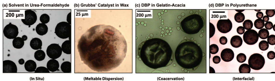
Figure 50. (a) Solvent-filled urea–formaldehyde (UF) capsules prepared by an in situ polymerization technique. (b) Grubbs' catalyst microspheres prepared by a meltable dispersion technique. (c) Dibutylphthalate (DBP)-containing gelatin–gum acacia microcapsules prepared by a coacervation technique. (d) DBP-containing polyurethane microcapsules produced using an interfacial polymerization technique. 367
