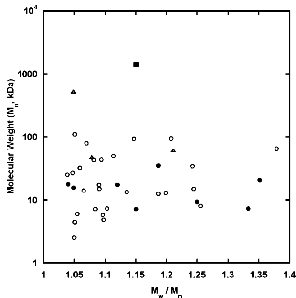
Figure 11. Molecular weight ( M_n ) vs PDI ( M_w/M_n ) for various living polymerizations: cationic ( \bullet ), anionic ( \circ ), and coordination catalysts ( \triangle ). 156 SET-LRP ( \blacksquare ) is shown for comparison. 160
