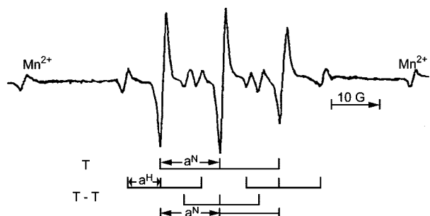
Figure 13. ESR spectrum observed at room temperature for a PMMA–benzene solution with added PMNB after 2 h of ultrasonic irradiation at 40 °C. Stick diagrams are also shown in which a^H and a^N (the hyperfine coupling constants) stand for separations due to coupling of the radical to a hydrogen and nitrogen nucleus. 178
